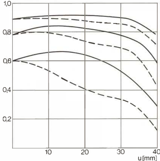
E Relative illuminance
