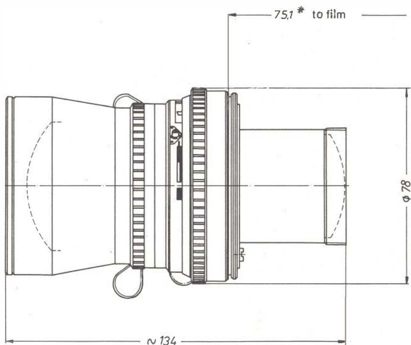
* flange focal distance with reseau
