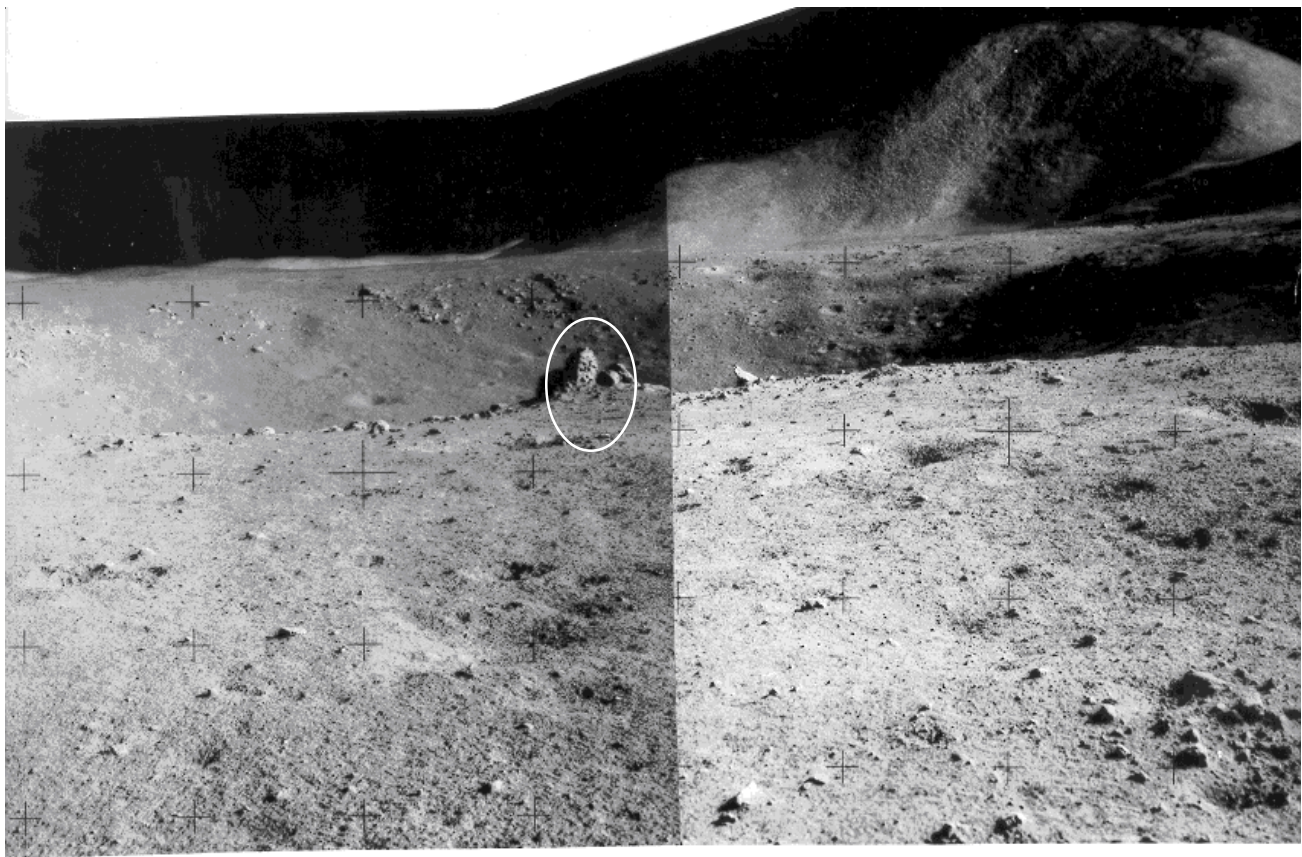
Figure 2: Dune crater Apollo 15. NASA S71-51736. Samples 15485, 15486 and 15499 were collected from the boulder in center of photo (on south rim). Hadley-Delta in the distance.
