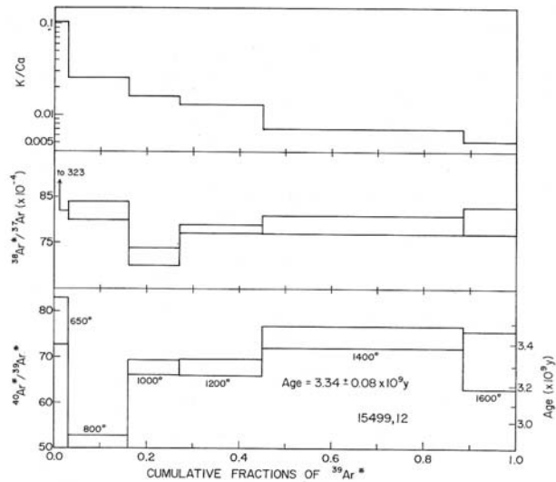
Figure 8: Ar/Ar plateau diagram for 15499 (Husain 1974).
