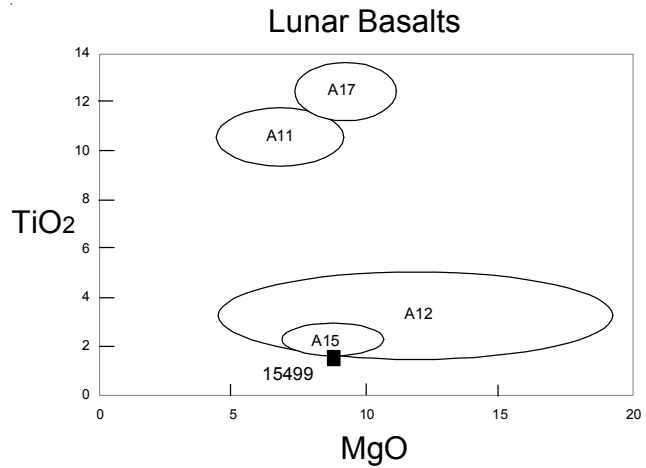
Figure 6: Chemical composition of 15499 compared with that of other lunar basalts.
