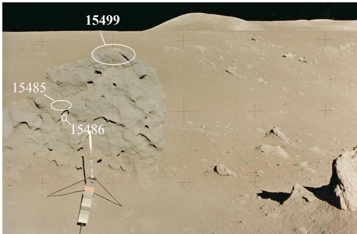
Figure 3: Boulder at Dune crater with location of samples. The feet on the gnonen are 50 cm apart. AS15-87-11768.
