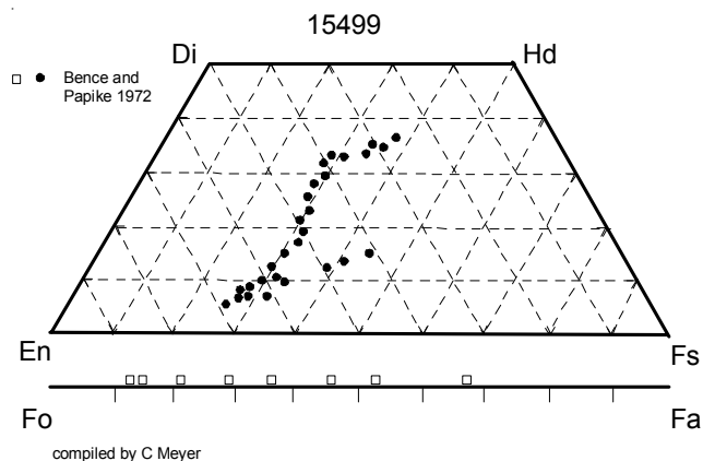
Figure 5: Composition of pyroxene in 15499 showing two Ca trends, dependent upon crystallographic direction (from Bence and Papike 1972). Also showing wide variation in composition of large, zoned, olivine grain.
